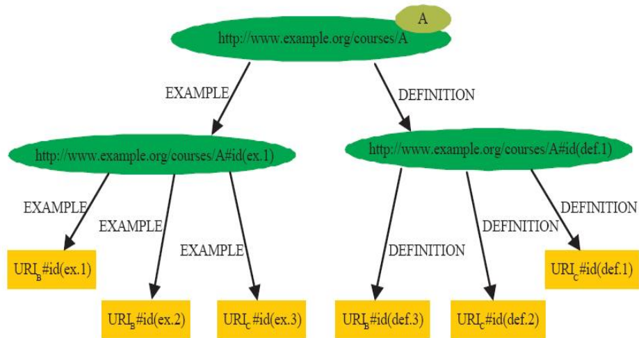
Figure 3: An example Relation Architecture
