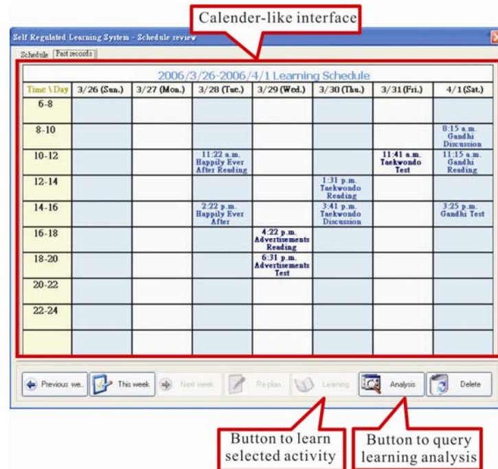
Figure 7. Learning review tool
