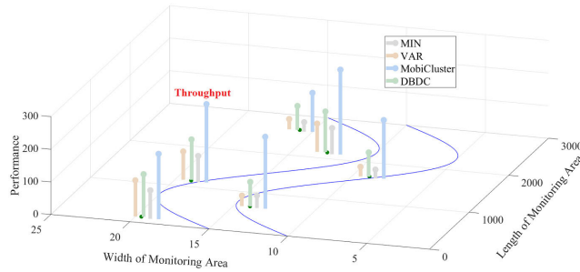
(a) Throughputs of selected 6 sensors in RCD scenario.
