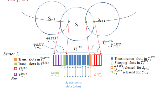
FIGURE 4. An example of case \beta_i = 1 .
