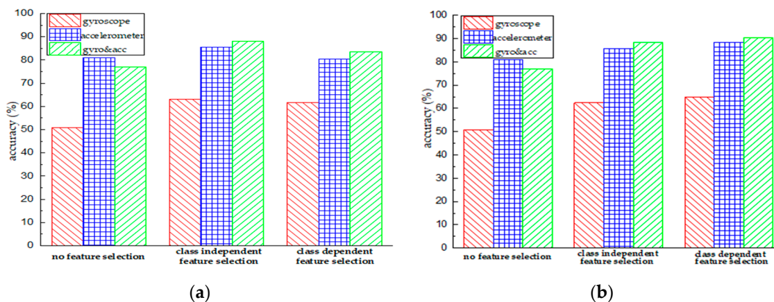
Figure 7. Performance comparison of using different sensing units in the case of no feature selection, class independent feature selection, and class dependent feature selection. (a) Performance obtained using the non-hierarchical model; (b) Performance obtained using the hierarchical model.
