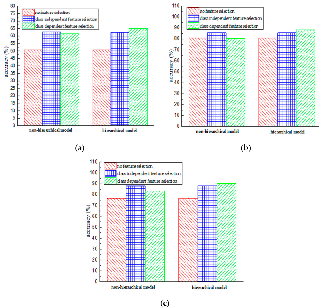
Figure 8. Performance comparison of using different feature selection methods in the case of the non-hierarchical model and hierarchical model. (a) Performance obtained using the gyroscope data; (b) Performance obtained using the accelerometer data; (c) Performance obtained using the accelerometer & gyroscope data.
