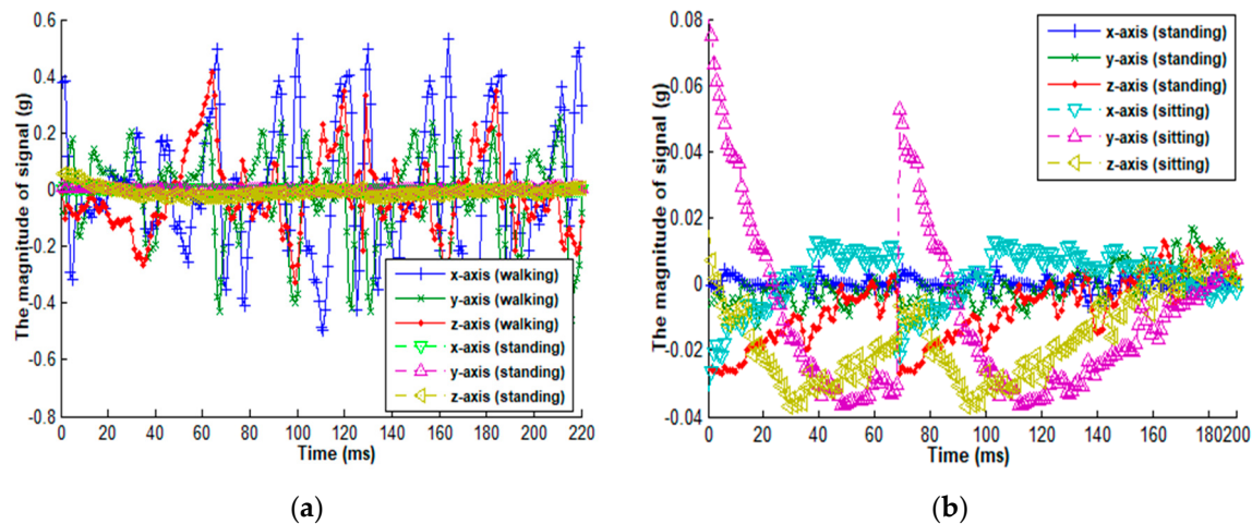
Figure 1. Comparison of the magnitude of a tri-accelerometer among three different activities. The accelerometer has sensor readings from three axes, i.e., x-axis, y-axis, and z-axis. (a) Comparison of walking and standing; (b) Comparison of standing and sitting.
