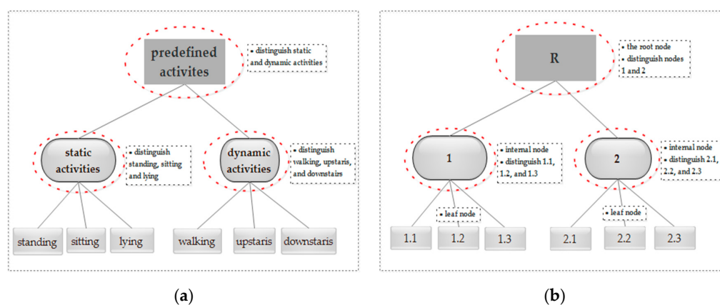
Figure 2. The proposed hierarchical activity recognition framework. The framework essentially organizes the predefined activities of interest into a hierarchical tree that indicates the relationship among different activities. (a) An example of a hierarchical activity recognizer; (b) Abstract form of the corresponding hierarchical structure.
