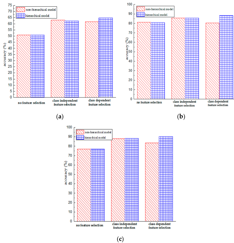
Figure 9. Performance comparison of using the non-hierarchical model and the hierarchical model in the case of no feature selection, class independent feature selection, and class dependent feature selection. (a) Performance obtained using the gyroscope data; (b) Performance obtained using the accelerometer data; (c) Performance obtained using the accelerometer & gyroscope data.
