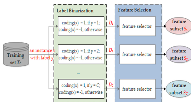
Figure 3. The proposed class dependent feature selection method. For a C -class problem, C feature subsets are finally returned, and they are probably different from each other.
