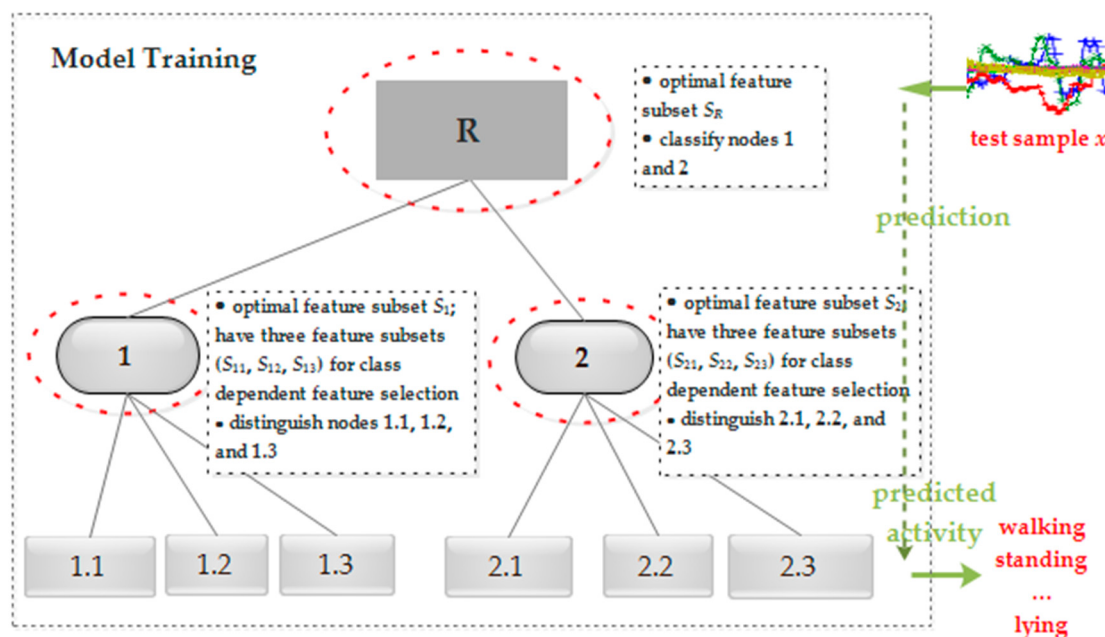
Figure 5. The proposed hierarchical activity recognition framework with feature selection integrated. In the phase of training, it selects the optimal feature subset and builds a classifier for each of the non-leaf nodes. In the phase of prediction, it adopts a top-down fashion to give the predicted label.
