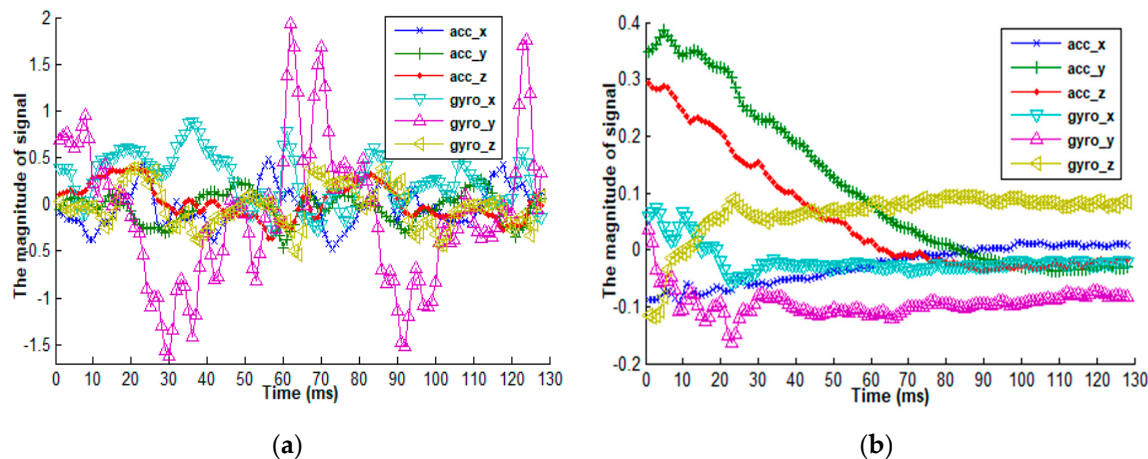
Figure 6. A comparison of the sensor readings between a tri-accelerometer and a tri-gyroscope when an individual is performing an activity. (a) The situation of going upstairs; (b) The situation of sitting.
