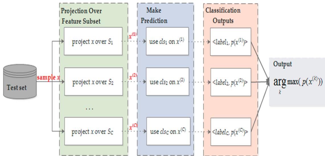
Figure 4. The scheme of classifying a test sample with the class dependent feature selection method. It first projects the test sample over different feature subsets, then uses the trained classifiers to make predictions, and finally determines the predicted label according to the maximal probability rule.
