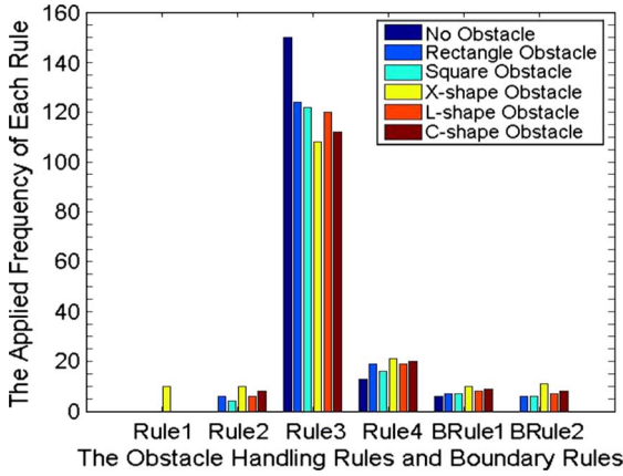
Fig. 24. Applied frequency of each rule proposed in ORRD in an environment containing a regular obstacle with various shapes.
