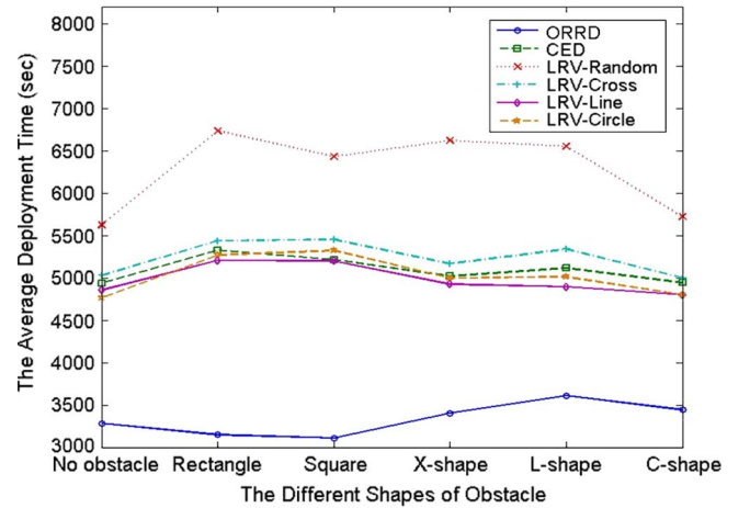
Fig. 21. Average deployment time after applying the ORRD, CED, and LRV in the environment containing multiple regular obstacles with different shapes.
