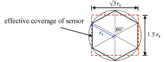
Fig. 11. Effective coverage region of hexagon deployment treated as a rectangle region that has the same area size as the hexagon region shown in Fig. 10(c).
