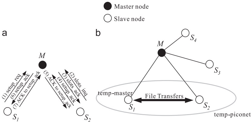
Fig. 1. The procedure of time-slot leasing.
