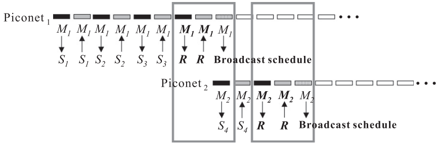
Fig. 10. Relay communication under scatternet.
