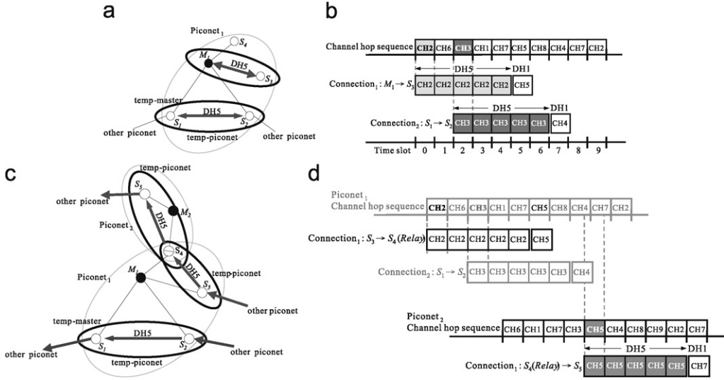
Fig. 4. The concept of overlapping communication scheme.
