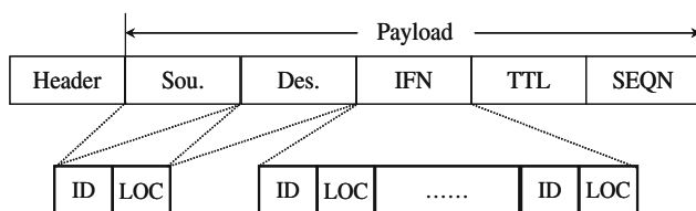
Fig. 3 Format of the Route Search Packet
