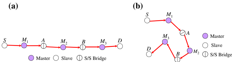
Fig. 14 The basic idea of route optimization. (a) The original topology of the route. (b) The new topology of the route
