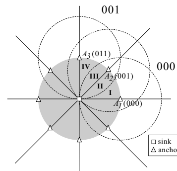
Figure 3. Anchor deployment strategy. All nodes in the shaded region are neighbors of the sink.
