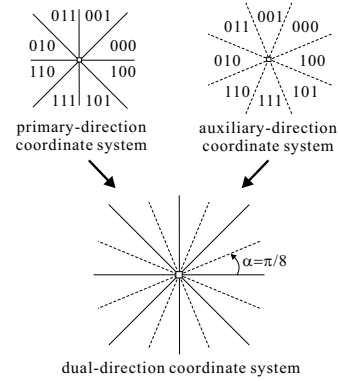
Figure 4. Dual-direction coordinate system with 8 directions.
