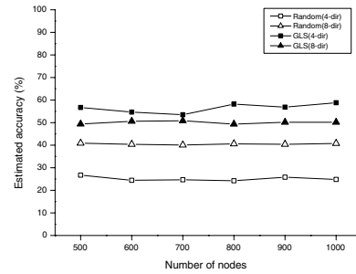
Figure 7. Estimated accuracy vs. number of nodes.
