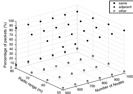
Figure 2. Experimental results for the impacts of the packets at a node.
