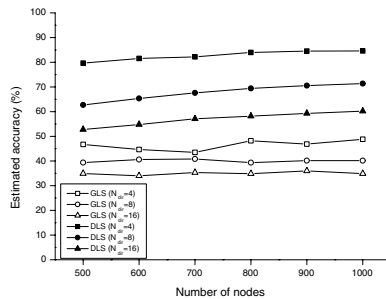
Figure 10. Estimated accuracy vs. number of nodes for GLS and DLS.
