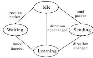
Figure 6. State transition diagram in DLS.
