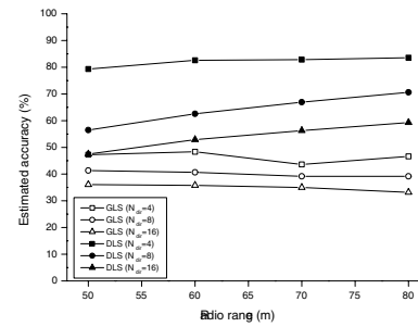
Figure 11. Estimated accuracy vs. radio range for GLS and DLS.
