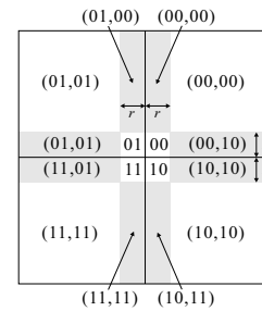
Figure 5. Coding system with 4 directions, where r is the radio range of a sensor node. All unknown nodes in the boundary error regions (namely, shaded regions) have two direction codes represented in the form (primary-direction code, auxiliary-direction code).
