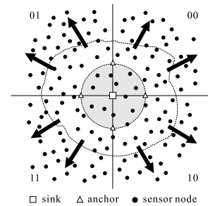
Figure 1. Basic concept of DLS.
