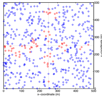
Figure 9. Example of the estimated result for 500 nodes scattered in the network with 4 directions. The blue and red nodes represent the accurate and erroneous estimates, respectively.
