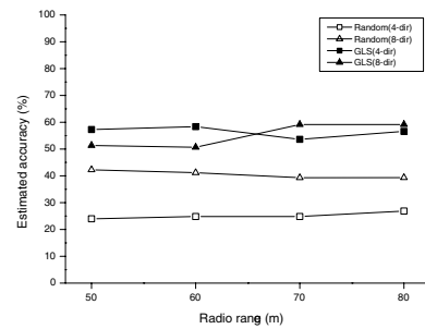
Figure 8. Estimated accuracy vs. radio range.
