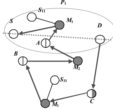
Figure 10. Route reply phase based on reduction and replacement rule.
