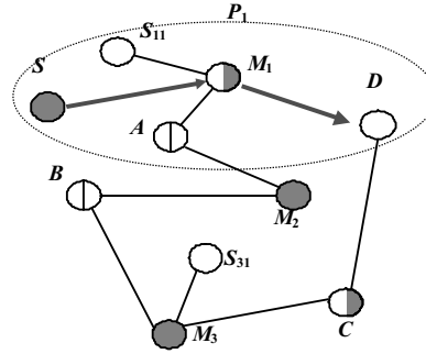
Figure 12. Final route construction phase in LARP.
