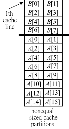
Figure 5. The nonequal-sized cache partitioning and mapping of arrays A and B for loop L2 .
