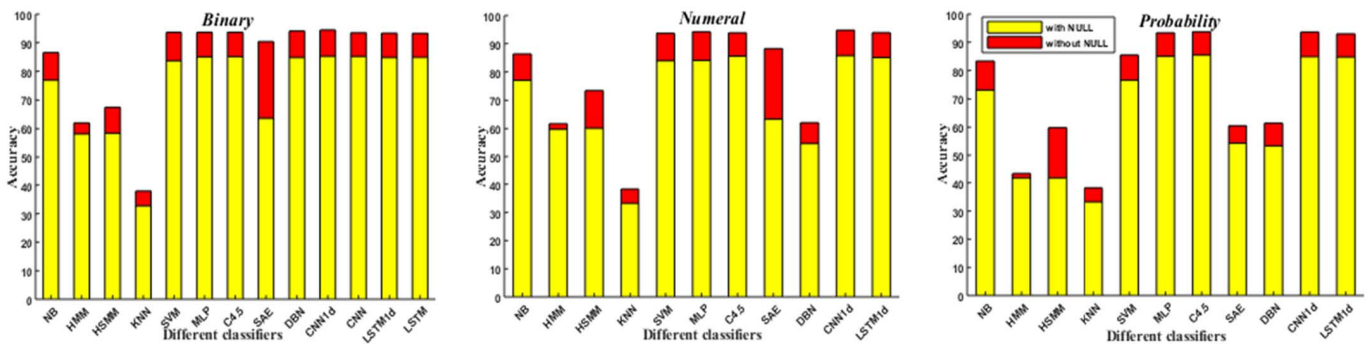
Fig. 6. Performance comparison between with and without NULL class on SH-a.
