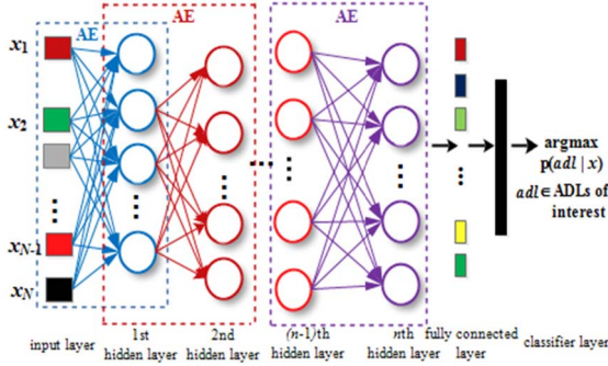
Fig. 2. SAE-based activity recognition model with environment sensors.
