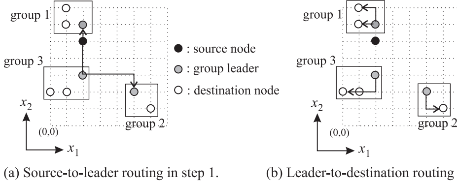
Figure 3: Multicast with proximity grouping by using Hamiltonian dual-path routing.
