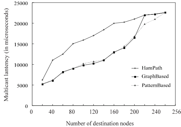
Figure 11: Comparison of Hamiltonian-path, graph-based and pattern-based proximity grouping schemes to destinations with proximity relations on 16 \times 16 mesh.
