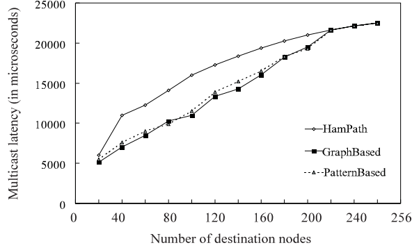
Figure 10: Comparison of Hamiltonian-path, graph-based and pattern-based proximity grouping schemes to random destinations on 16 \times 16 mesh.
