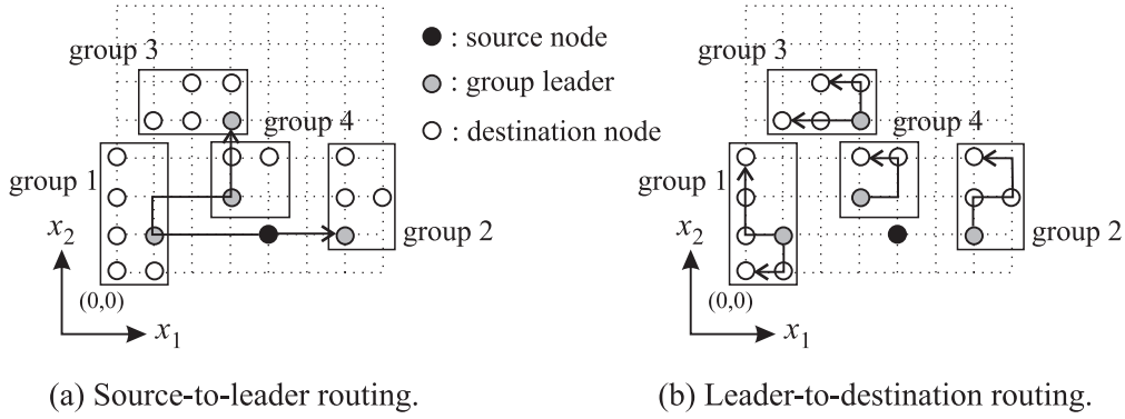
Figure 9: Multicasting via pattern-based proximity grouping by using Hamiltonian dual-path routing.
