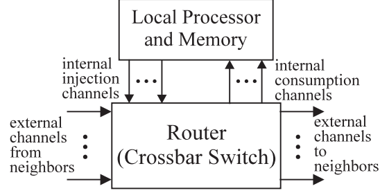
Figure 1: A node architecture with multidestination routing.
